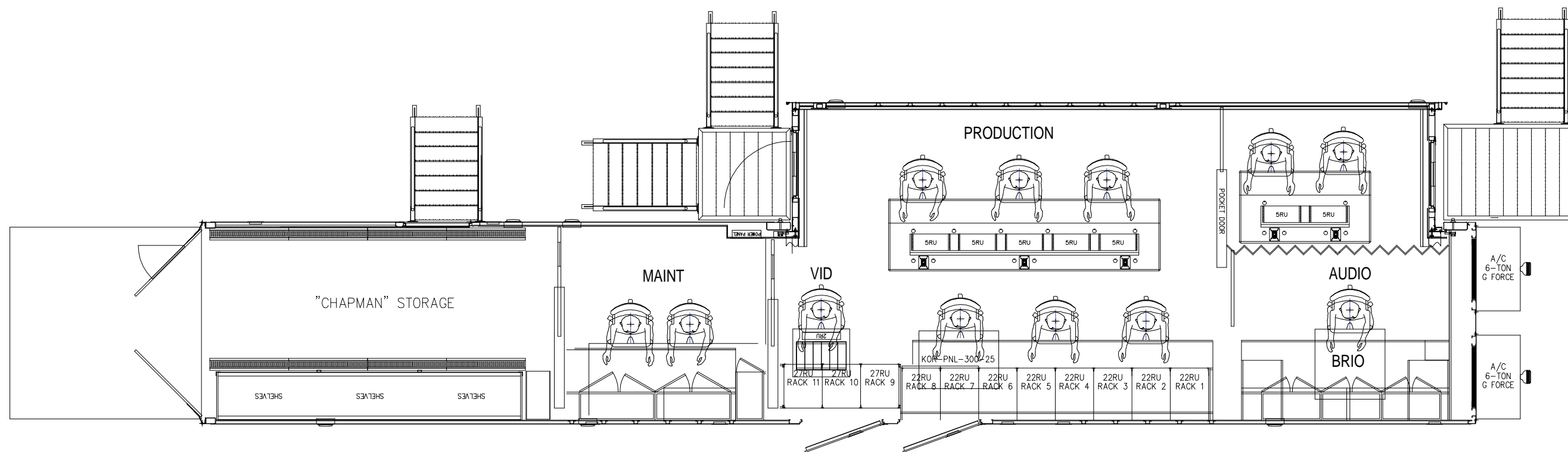
GCV PRIDE B DUAL FEED CONFIG.
