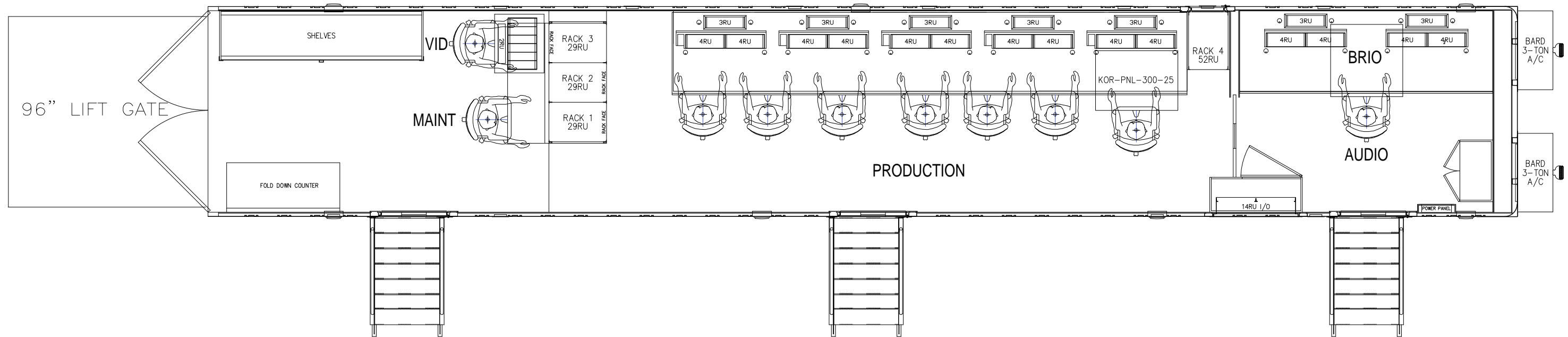
GCV B-1 DUAL FEED CONFIG.
